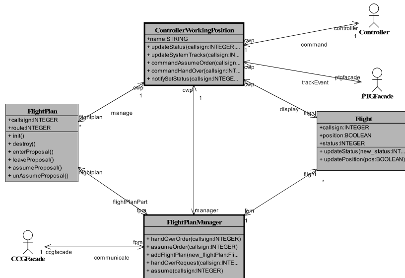
Figure 6-4: The class diagram of the ATC application example.
