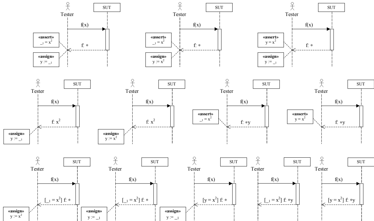
Figure 4-8: Twelve alternative syntaxes for the same behaviour showing the use of assign and assert internal actions attached to SUT-message arrowheads, proper-reception assigned variables, anonymous variables, and guards.
