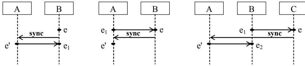
Figure 5-5: The extra causality relations of Fig 5-3 implemented via synchronization messages
