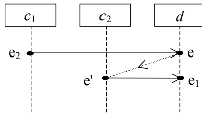
Figure 5-7: Illustration of the extra immediate-causality relations described in rule 3a
