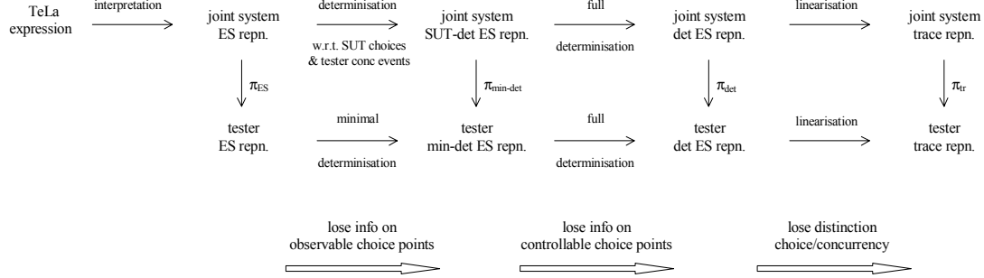
Figure 3-4: Part of the spectrum of possible semantics.
