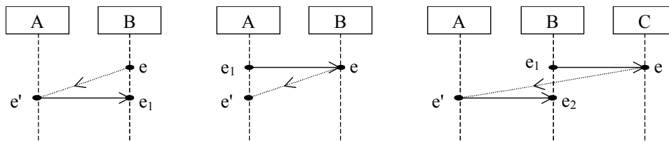
Figure 5-3: Illustration of the extra immediate-causality relations added by the relation << w.r.t. the relation \leq
