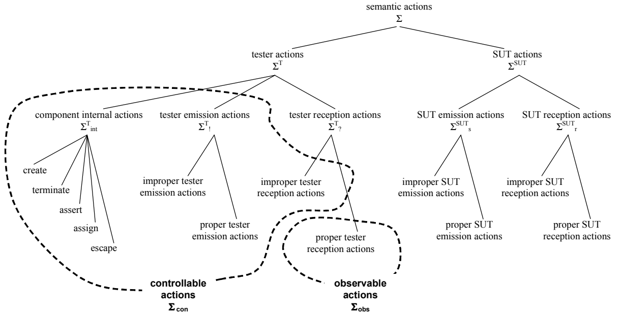
Figure 5-1: The set of actions of TeLa. The semantics after projection contains only the tester actions: those of the left branch.
